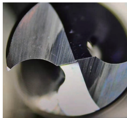
After grinding
