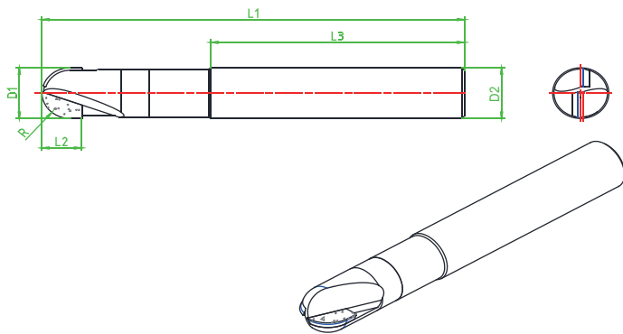
PCD ball nose mill-- Metric
