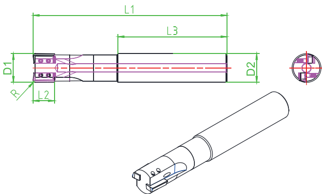
PCD quick change milling cutter-- Metric
