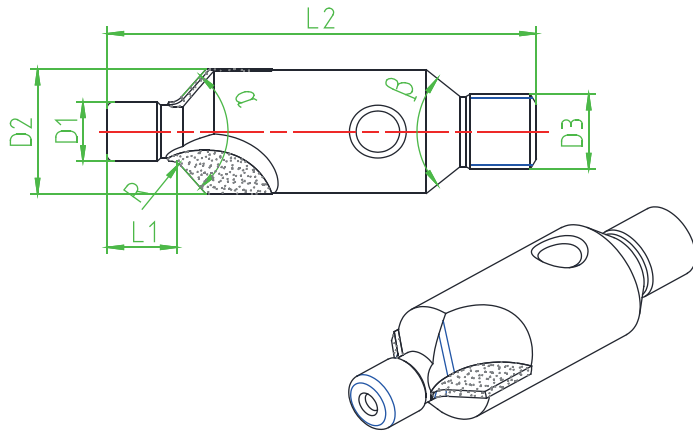
PCD socket drill-- Metric
