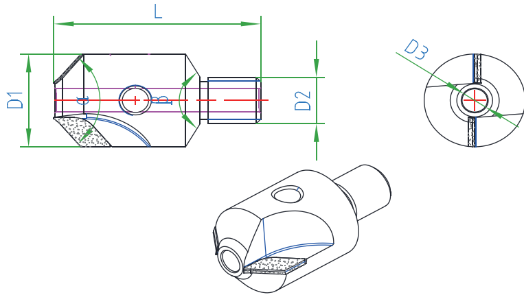
PCD socket drill with pin hole—Imperial
