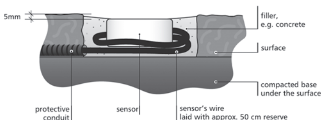
Example of temperature and moisture sensor's installation in the surface
