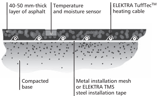
Cross section of a driveway or road with asphalt surface
